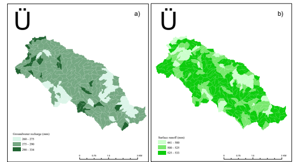
Sample SWAT model of Robit watershed, Ethiopia
